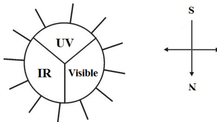
TRIBE (Electromagnetic Spectrum)
